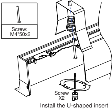
Install the U-shaped insert
