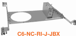
C6-NC-RI-J-JBX 18.5" W x 9" D x 4" H 6.25" Hole 14.25" Min. Extend 25" Max. Extend (Assembly Required)
