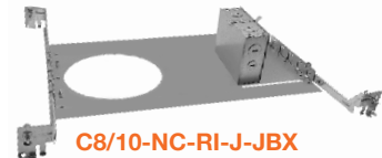
C8/10-NC-RI-J-JBX 18.5" W x 12" D x 4" H 8" Hole 14" Min. Extend 25" Max. Extend (Assembly Required)
