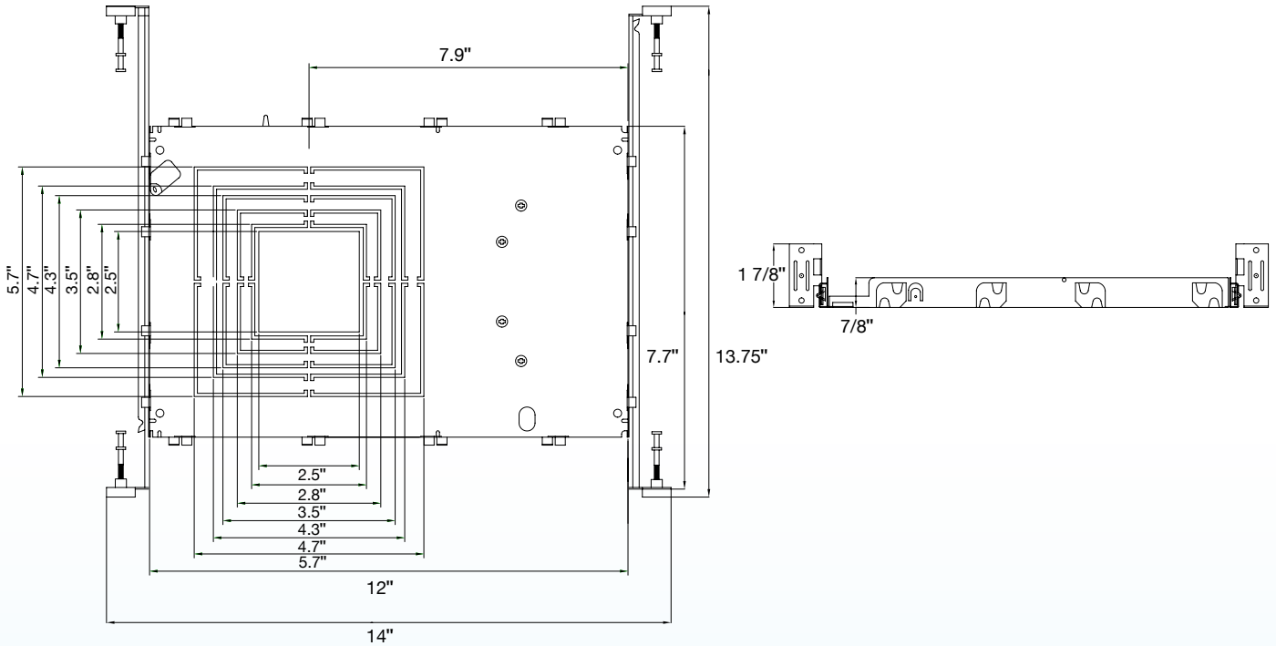
CUNV-NC-ICAT-6SQ Universal Mounting Plate
