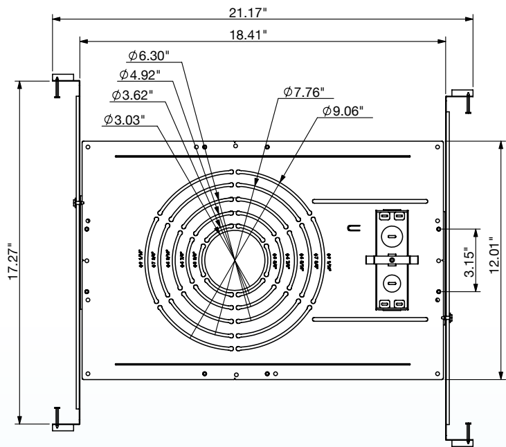
CUNV-NC-RI-J-JBX Universal Mounting Plate • Assembly Required
