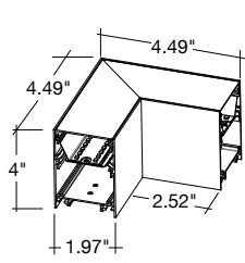
LED-ALIN2-L-D-5CCT-WH
