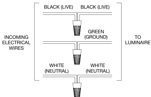
WIRING DIAGRAM 1
