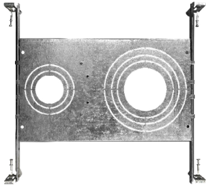
CUNV-NC-ICAT-7H Universal Pre-Mounting Plate 13 7/8" x 15 1/8"
