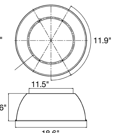
Aluminum Reflector
