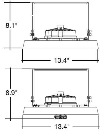
Surface Mount
