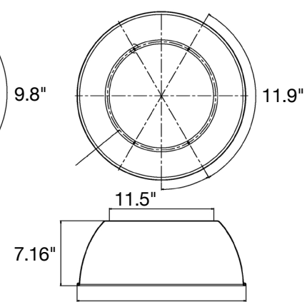
Aluminum Reflector
