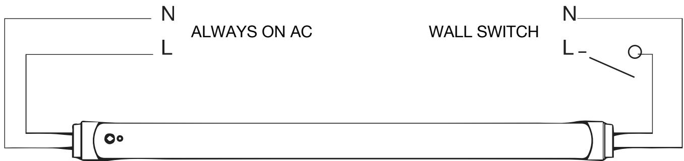
LED Tube Wiring Schematic
